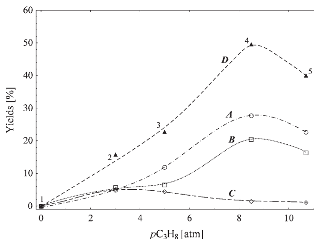
Figure 1. Effect of the \text{C}_3\text{H}_8 pressure on the yields of isobutyric (curve A ), n -butyric (curve B ) and acetic (curve C ) acids and on the total yield (curve D ) for the propane carboxylation catalysed by complex 1 ( p\text{CO}=20 atm). Reaction conditions and point numbers are those of the Table 1 entries.
