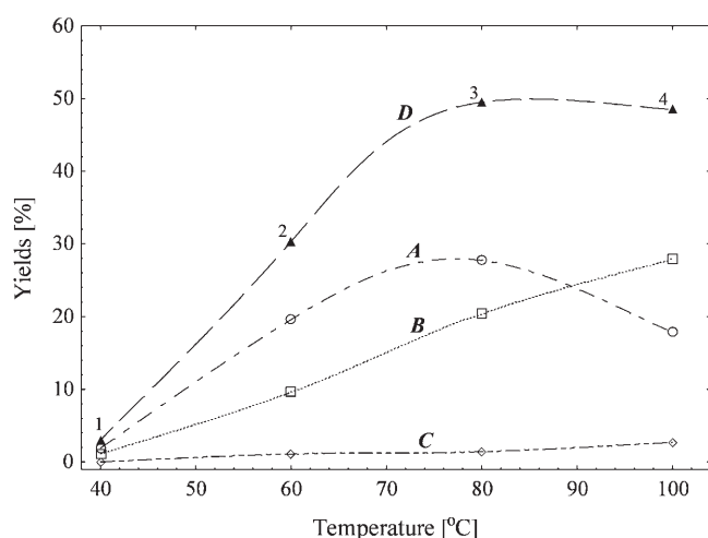
Figure 3. Effect of the temperature on the yields of isobutyric (curve A ), n -butyric (curve B ) and acetic (curve C ) acids and on the total yield (curve D ) for the propane carboxylation catalysed by complex 1 ( p_{\text{C}_3\text{H}_8} = 8.5 atm, p_{\text{CO}} = 20 atm). Reaction conditions and point numbers are those of the Table 3 entries.
