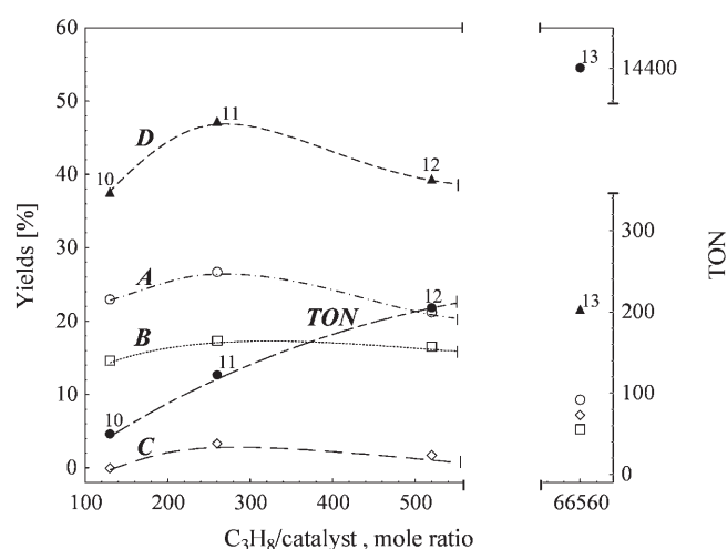
Figure 7. Effect of the catalyst 3 amount on the overall TON (points ●) and on the yields of isobutyric (curve A , points ○), n -butyric (curve B , points □) and acetic (curve C , points ◇) acids and on the total yield (curve D , points ▲) for the propane carboxylation ( p_{\text{C}_3\text{H}_8}=8.5 atm, p_{\text{CO}}=20 atm). Reaction conditions and point numbers are those of the Table 5 entries.
