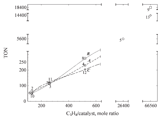
Figure 8. Effect of the catalyst amount on the TON for the propane carboxylation ( p_{\text{C}_3\text{H}_8}=8.5 atm, p_{\text{CO}}=20 atm) catalysed by complex 1 (curve A , points ○), 2 (curve B , points □), 3 (curve C , points ◇). Reaction conditions and point numbers are those of the Table 5 entries.
