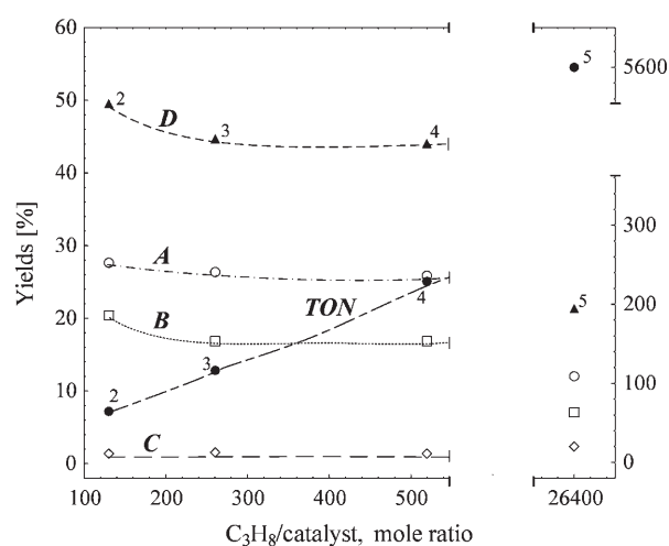
Figure 5. Effect of the catalyst 1 amount on the overall TON (points ●) and on the yields of isobutyric (curve A , points ○), n -butyric (curve B , points □) and acetic (curve C , points ◇) acids and on the total yield (curve D , points ▲) for the propane carboxylation ( p C 3 H 8 =8.5 atm, p CO=20 atm). Reaction conditions and point numbers are those of the Table 5 entries.
