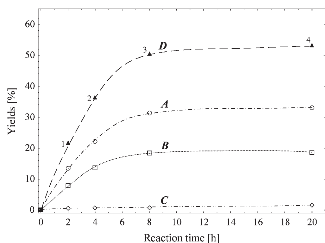
Figure 4. Effect of the reaction time on the yields of isobutyric (curve A), n -butyric (curve B) and acetic (curve C) acids and on the total yield (curve D) for the propane carboxylation catalysed by complex 1 ( p C 3 H 8 =8.5 atm, p CO=30 atm). Reaction conditions and point numbers are those of the Table 4 entries.
