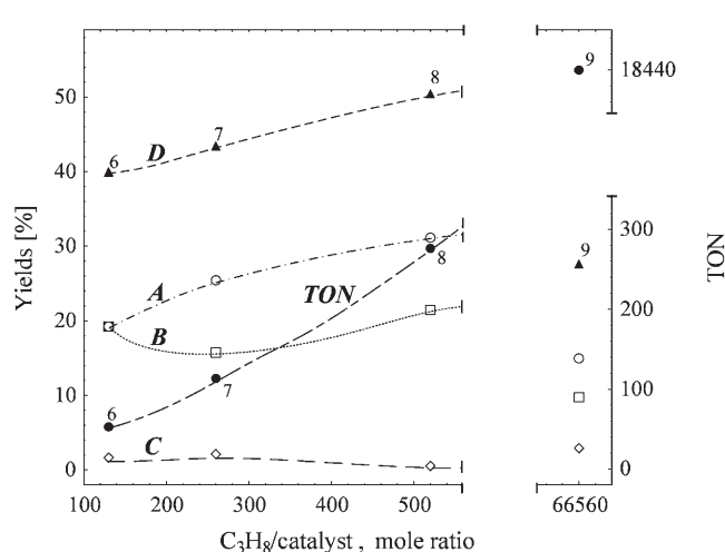
Figure 6. Effect of the catalyst 2 amount on the overall TON (points ●) and on the yields of isobutyric (curve A , points ○), n -butyric (curve B , points □) and acetic (curve C , points ◇) acids and on the total yield (curve D , points ▲) for the propane carboxylation ( p C 3 H 8 =8.5 atm, p CO=20 atm). Reaction conditions and point numbers are those of the Table 5 entries.
