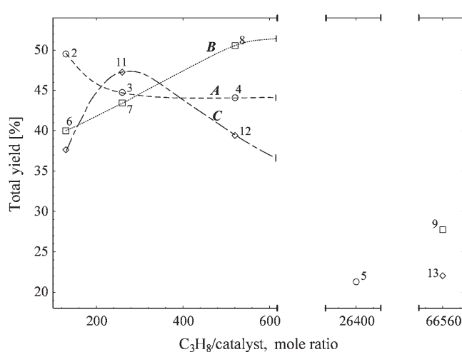
Figure 9. Effect of the catalyst amount on the total yield of carboxylic acids for the propane carboxylation ( p_{\text{C}_3\text{H}_8}=8.5 atm, p_{\text{CO}}=20 atm) catalysed by complex 1 (curve A , points ○), 2 (curve B , points □), 3 (curve C , points ◇). Reaction conditions and point numbers are those of the Table 5 entries.
